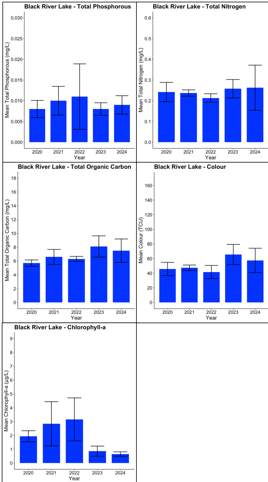
Figure 22. Black River Lake Phosphorus, Nitrogen, Organic Carbon, Colour, & Chlorophyll a graphs. Figures representing annual averages from the samples collected in Black River Lake between 2020 - 2024 including Total Phosphorous (Top Left), Total Nitrogen (Top Right), Total Organic Carbon (Middle Left), colour (Middle Right), and Chlorophyll-A (Bottom Left). Standard Deviation indicated by black bars.
