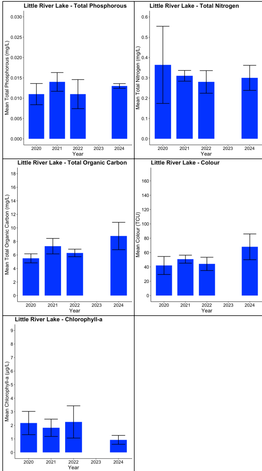
Figure 20. Little River Lake Phosphorus, Nitrogen, Organic Carbon, Colour, & Chlorophyll a graphs. Figures representing annual averages from the samples collected in Little River Lake between 2020 - 2024 including Total Phosphorous (Top Left), Total Nitrogen (Top Right), Total Organic Carbon (Middle Left), colour (Middle Right), and chlorophyll a (Bottom Left). Standard Deviation indicated by black bars.
