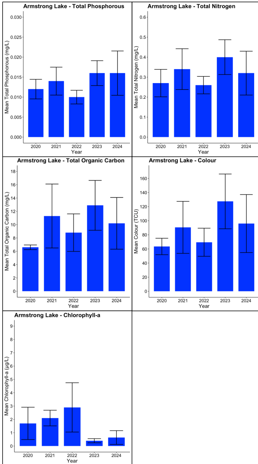
Figure 4. Armstrong Lake Phosphorus, Nitrogen, Organic Carbon, Colour, & Chlorophyll a graphs. Figures represent annual averages from the samples collected in Armstrong Lake between 2020 - 2024 including Total Phosphorous (Top Left), Total Nitrogen (Top Right), Total Organic Carbon (Middle Left), colour (Middle Right), and chlorophyll a (Bottom Left). Standard Deviation indicated by black bars.
