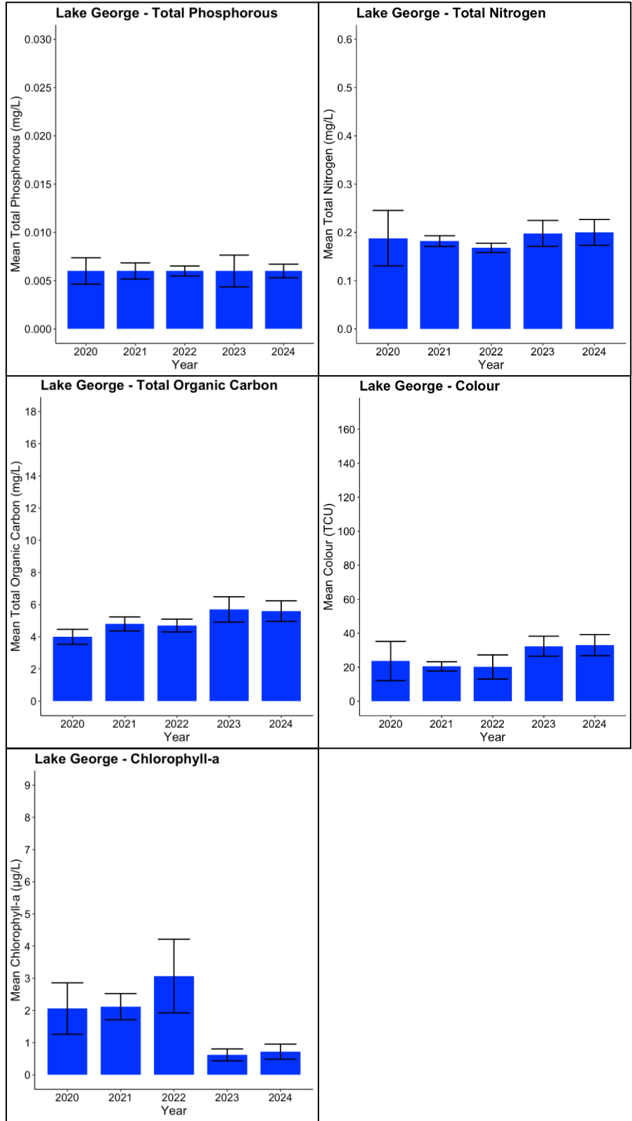
Figure 10. Lake George Phosphorus, Nitrogen, Organic Carbon, Colour, & Chlorophyll a graphs. Figures representing annual averages from the samples collected in Lake George between 2020 - 2024 including Total Phosphorous (Top Left), Total Nitrogen (Top Right), Total Organic Carbon (Middle Left), colour (Middle Right), and chlorophyll a (Bottom Left). Standard Deviation indicated by black bars.
