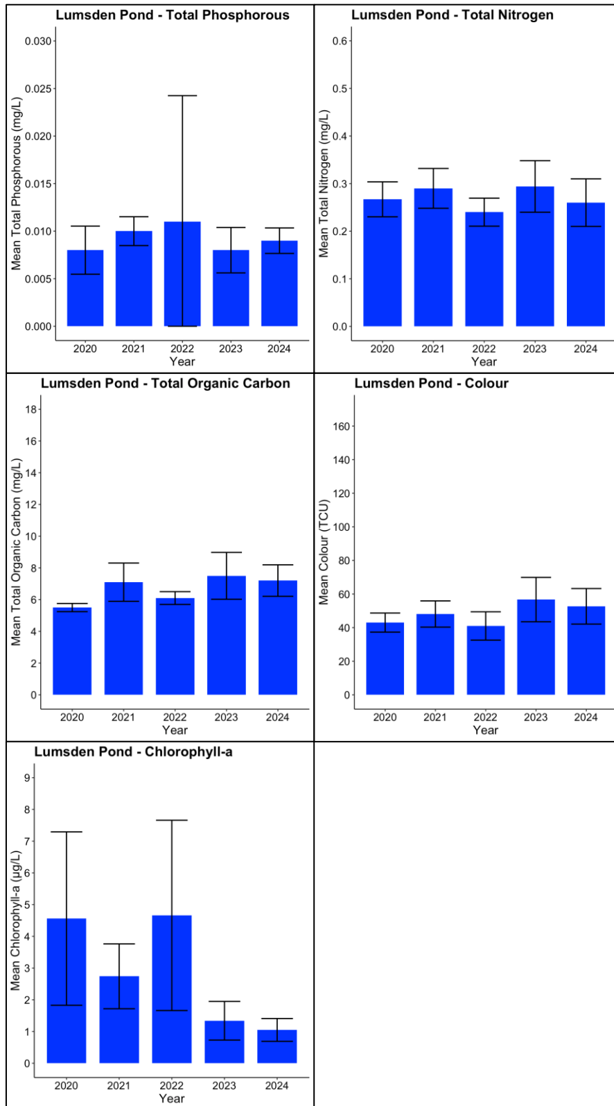
Figure 24. Lumsden Pond Phosphorus, Nitrogen, Organic Carbon, Colour, & Chlorophyll a graphs. Figures representing annual averages from the samples collected in Lumsden Pond between 2020 - 2024 including Total Phosphorous (Top Left), Total Nitrogen (Top Right), Total Organic Carbon (Middle Left), colour (Middle Right), and chlorophyll a (Bottom Left). Standard Deviation indicated by black bars.
